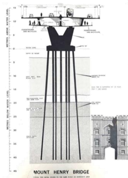
Engineering sketch of Mount Henry Bridge 1 (1982) Source: HCWA State Register Place entry, 2026 (Courtesy of Main Roads WA, showing depth of piles driven into the riverbed, and using Barracks Arch as scale)
