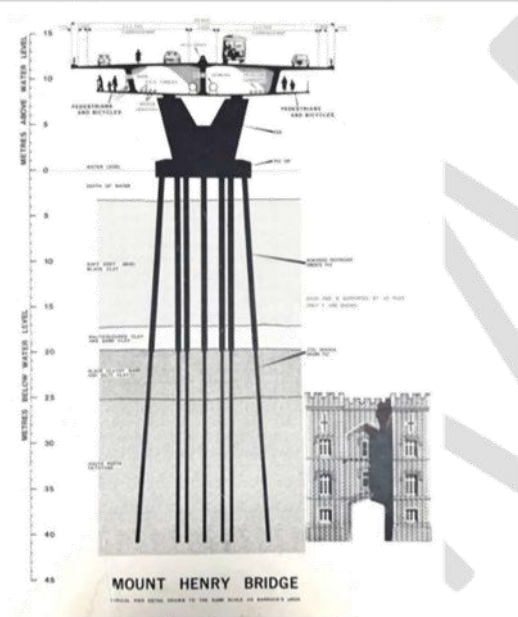
Engineering sketch of Mount Henry Bridge 1 (1982) Source: HCWA State Register Place entry, 2026 (Courtesy of Main Roads WA, showing depth of piles driven into the riverbed, and using Barracks Arch as scale)
