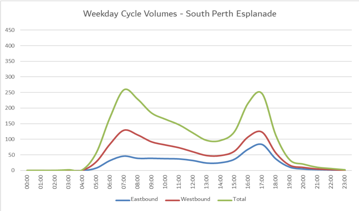
Figure 68 Weekday cycle volumes South Perth Esplanade 2020/2021
