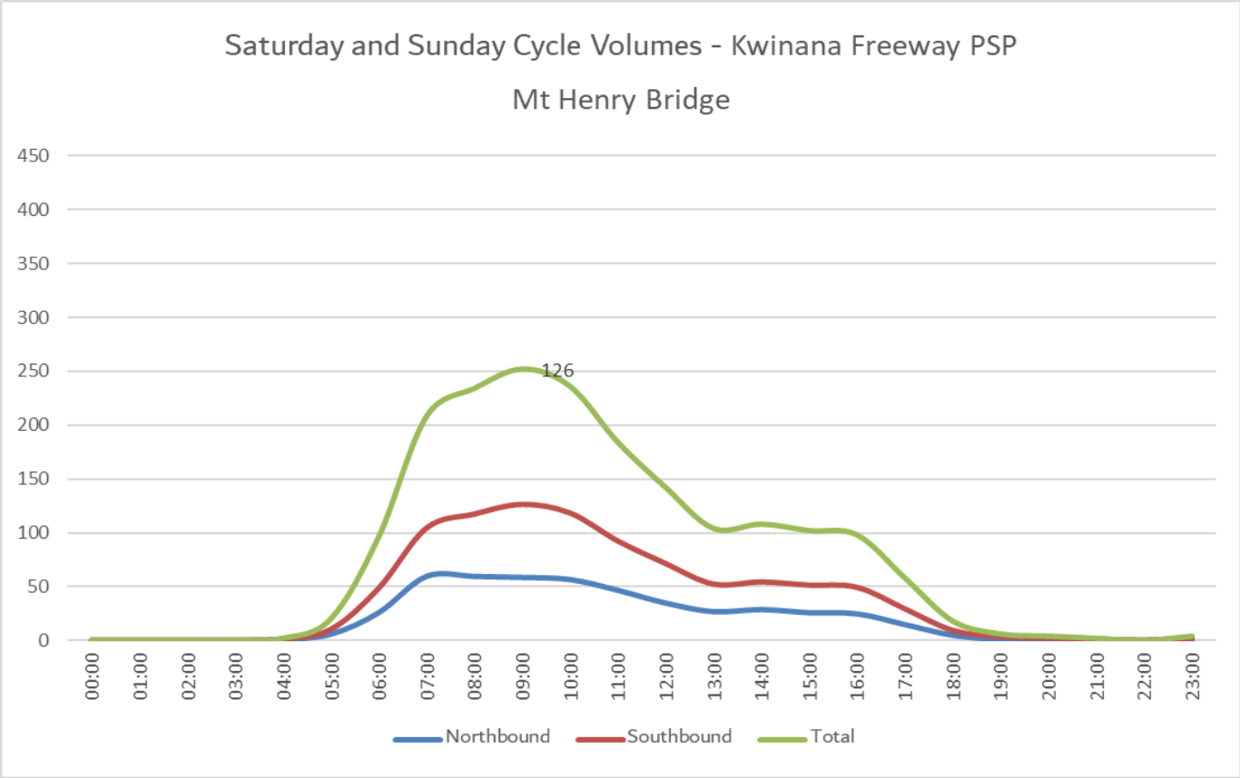
Figure 69 Weekend cycle volumes Kwinana Freeway PSP 2020/2021
