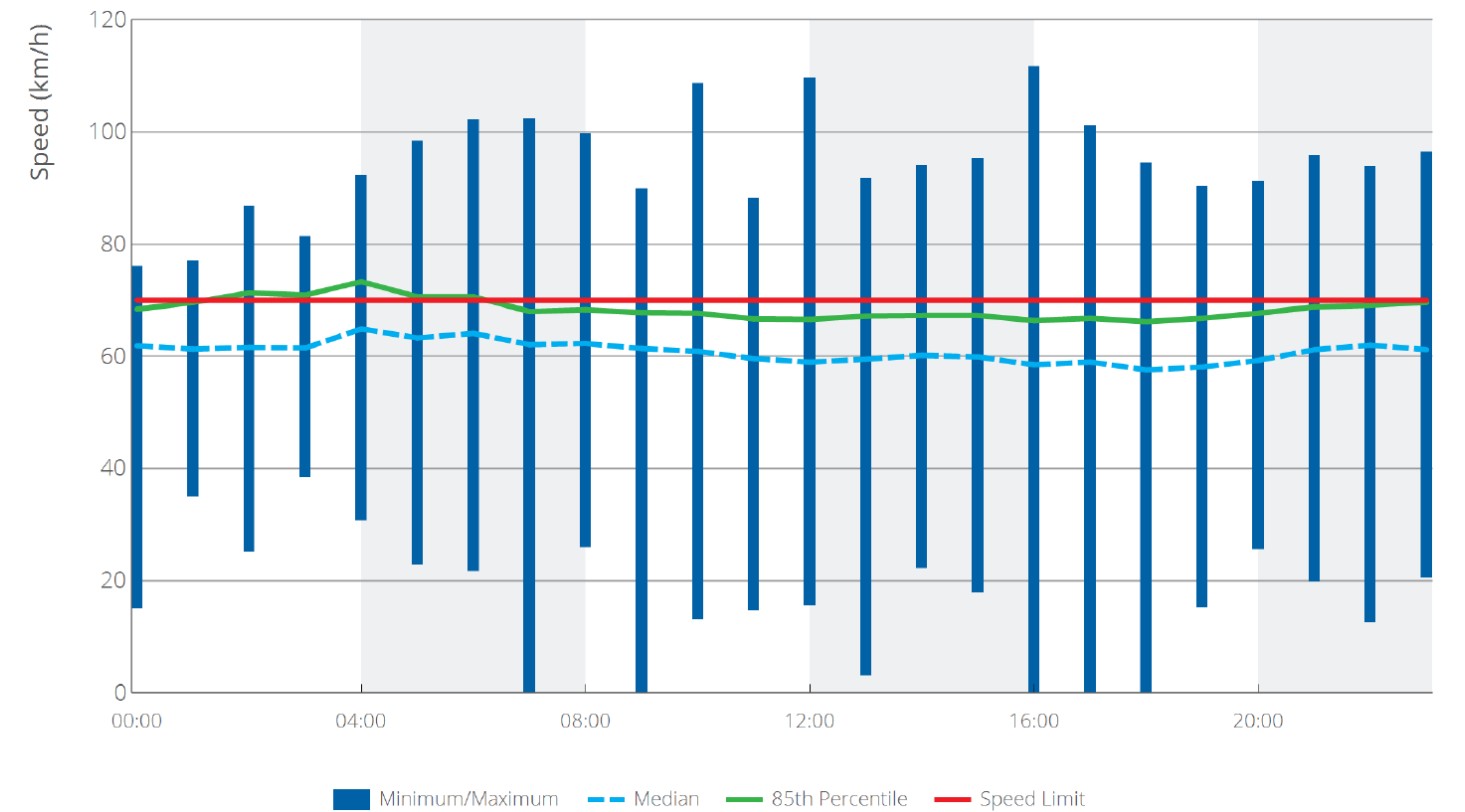
Figure 43 Speed profile Kent Street north of Manning Road 2018
