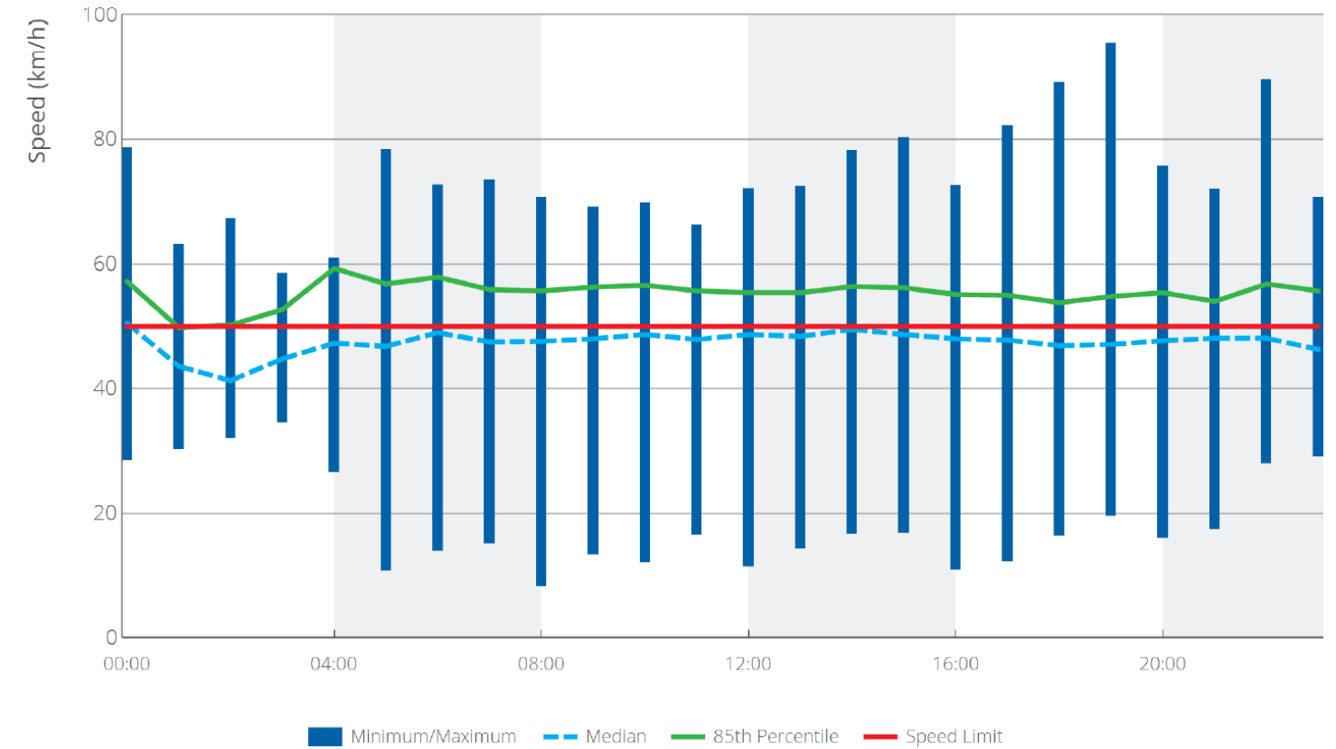
Figure 56 Speed profile Waterford Avenue south of Manning Road
