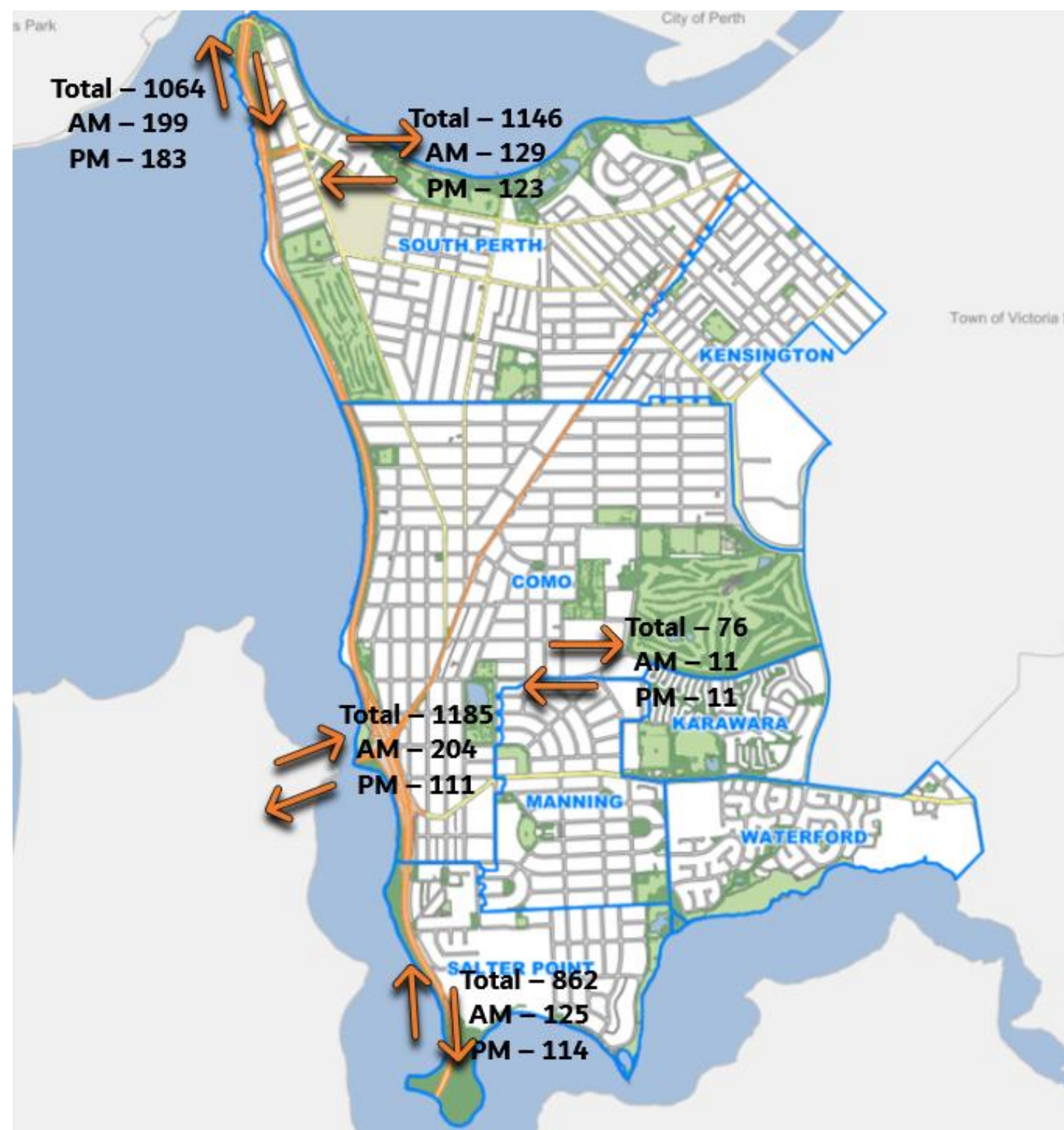
Figure 70 Weekday cycle volumes (source: MRWA TrafficMap)
