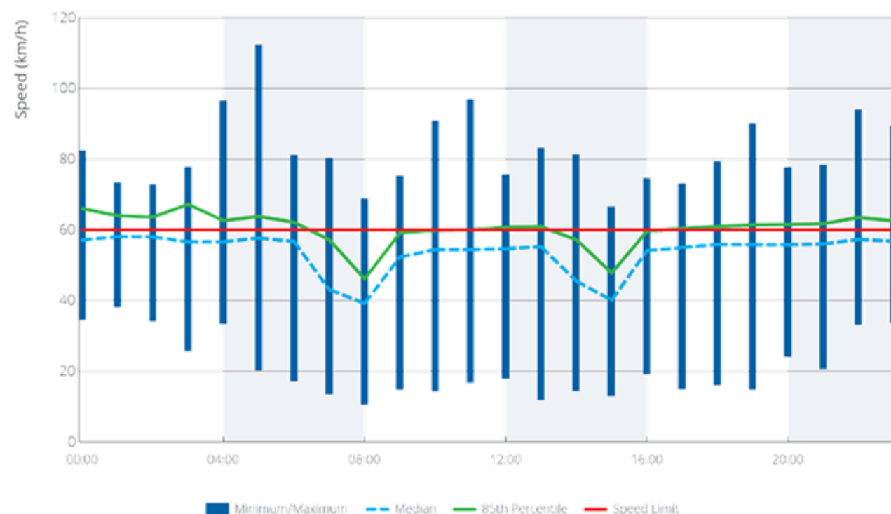
Figure 41 Speed profile George Street south of Baron Hay Court
