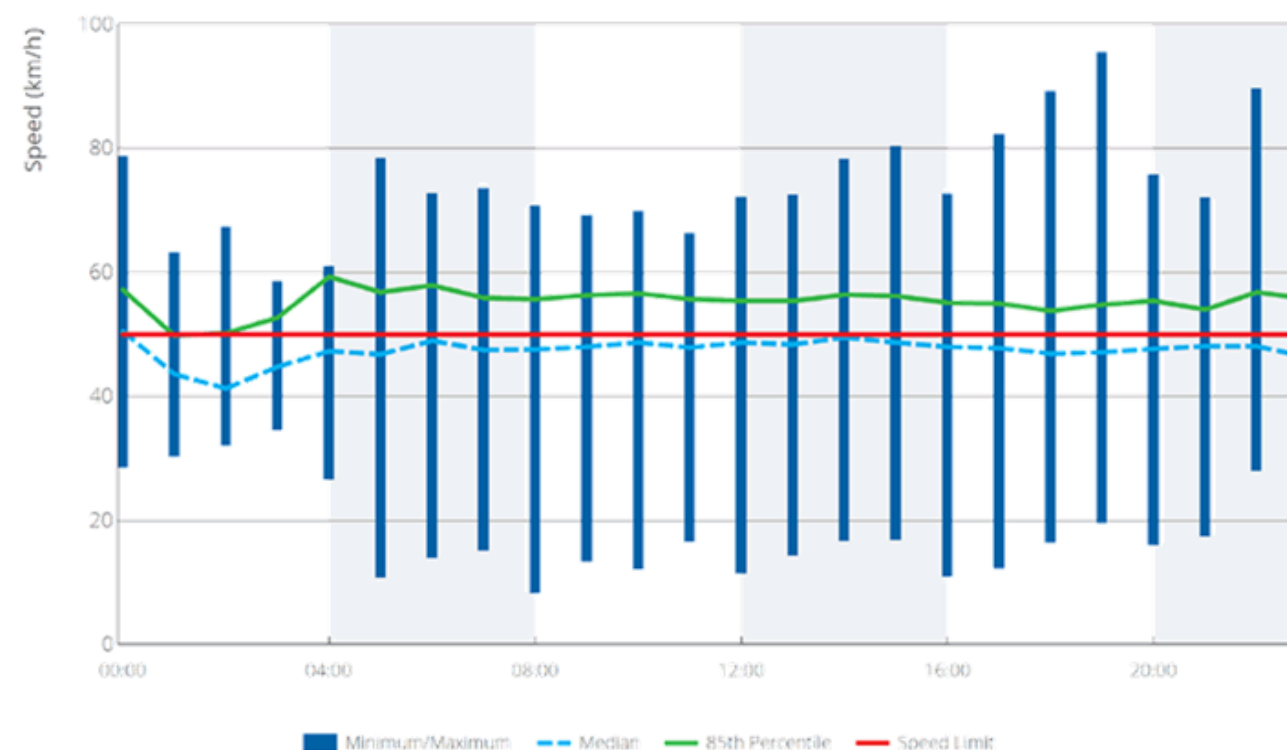
Figure 56 Speed profile Waterford Avenue south of Manning Road
