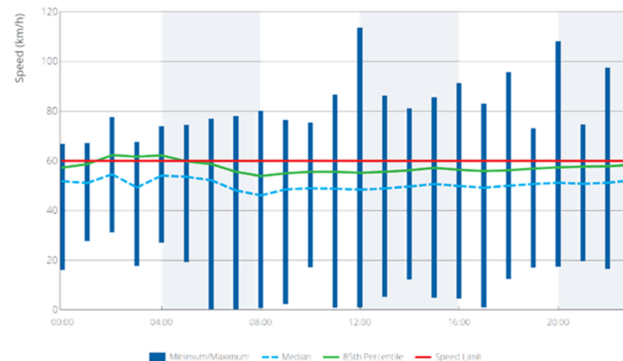
Figure 45 Speed profile Labouchere Road south of Judd Street 2018
