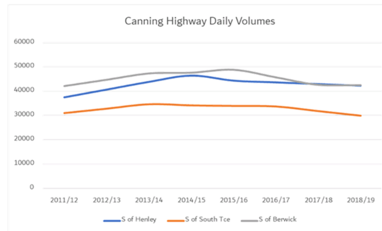
Figure 79 - Canning Highway historic count data
