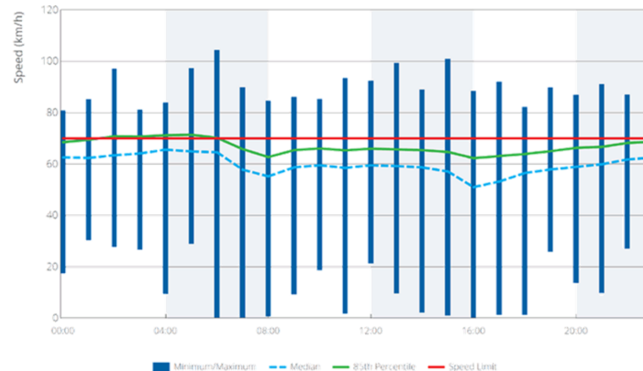
Figure 48 Speed profile Manning Road west of Centenary Avenue 2018
