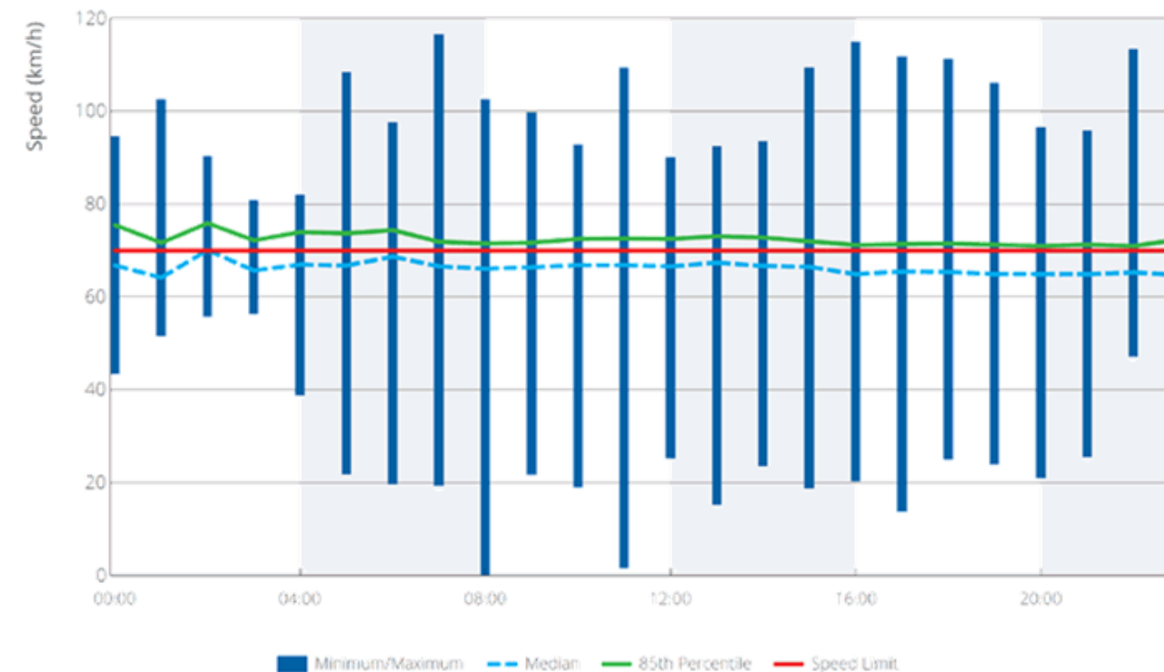
Figure 42 Speed profile Hayman Road south of South Terrace 2018
