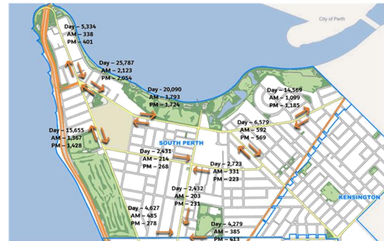
Figure 3 Distributor road volumes - South Perth
