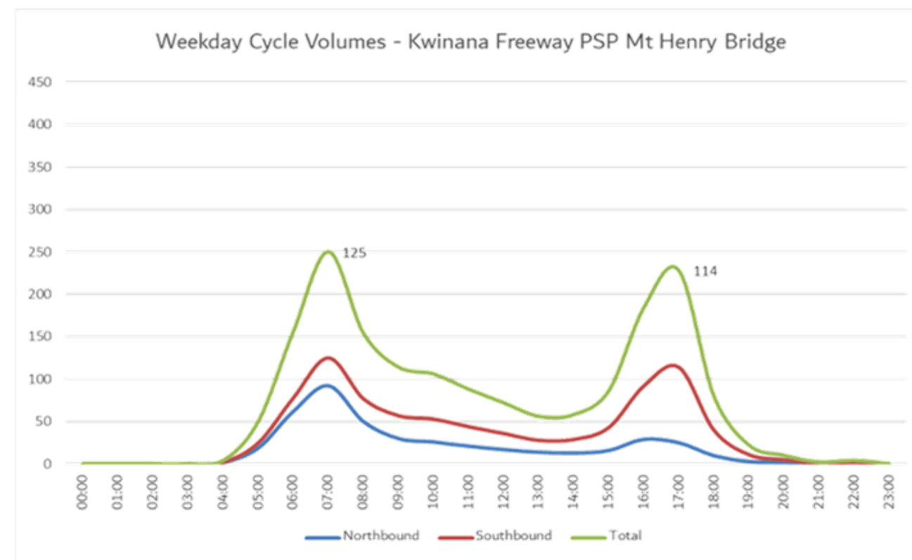
Figure 66 Weekday cycle volumes Kwinana Freeway PSP Mt Henry Bridge 2020/2021
