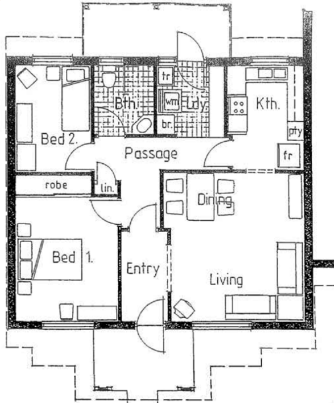
Plan Unit 'B' adapted
